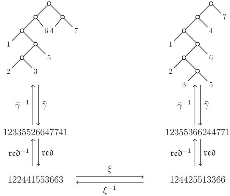
Figure 5.3: Example of the bijections \tilde{\gamma} , \mathbf{red} and \xi
