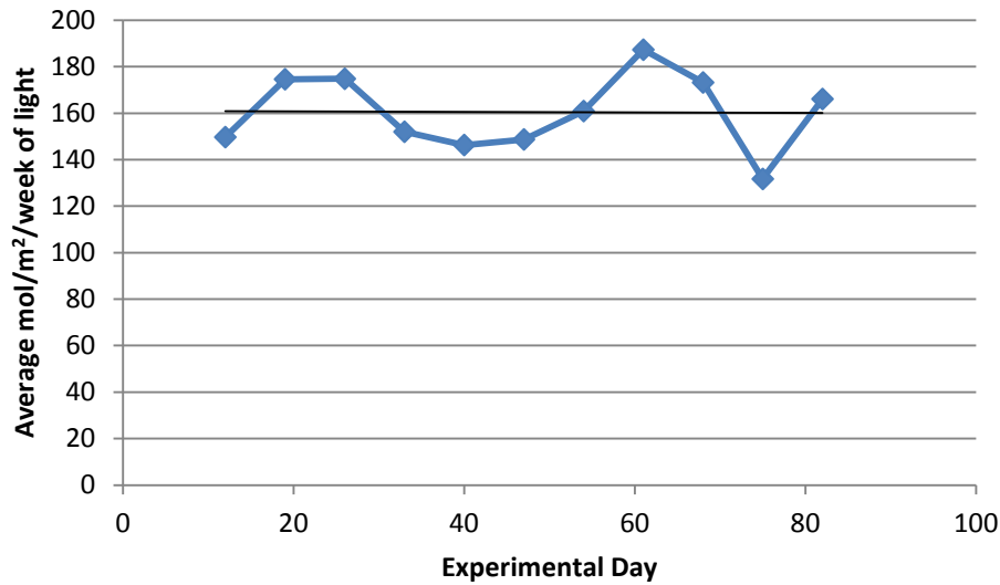
Figure 3: Light levels reaching coral tanks, measured over the course of the experimental period and reported as the average mol/m 2 /week. Light levels were stable throughout the experiment ( y = -0.0119x + 161.04 , p = 0.85 ).
