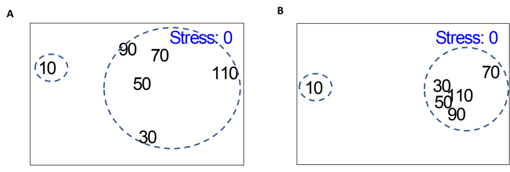
Figure 2.2. Nonmetric multidimensional scaling (MDS) plots revealing that samples nearest the mangroves separate from the rest in both the dry (A) and wet (B) season. Dashed lines indicate cluster analysis grouping of samples at about 80 % similarity. Numerical values indicate distance from the mangrove-seagrass shoreline. Success of MDS is measured by a stress coefficient. Stress < 0.05 gives an excellent representation with no prospect for misinterpretation.
