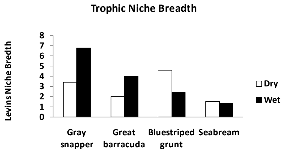
Figure 3.4. Levins' index of trophic niche breadth calculated for gray snapper, seabream, bluestriped grunt and great barracuda in Biscayne Bay, Florida (USA). Dietary niche breadth values were calculated on the percent by volume contribution of different food items in fish diets.
