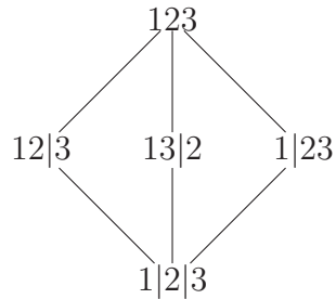
Figure 1.1: \Pi_3
